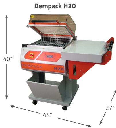
Dempack H20 shown with a trim collection bin option
